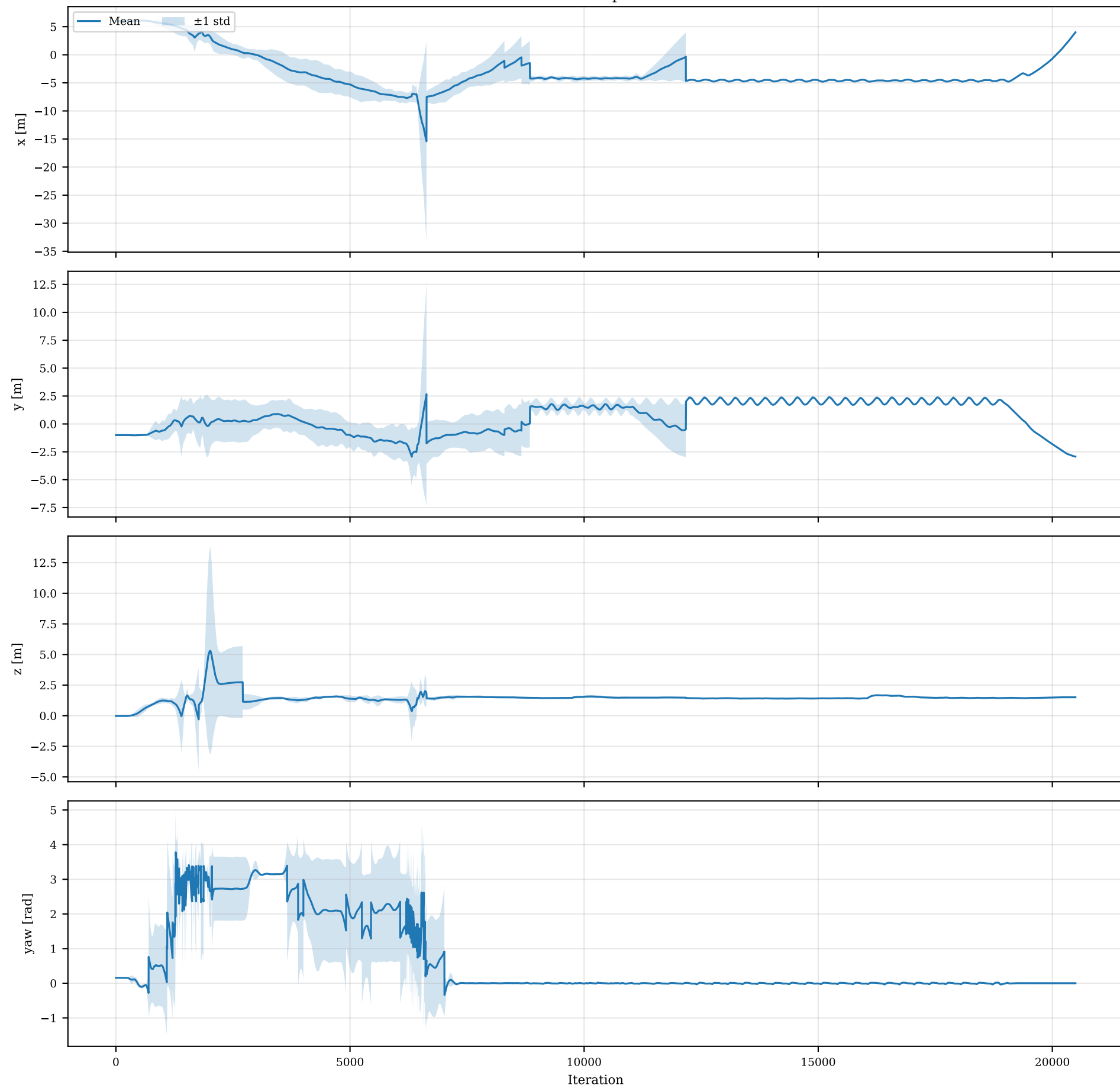
5 UAVS - UAV 32 - Mean position \pm std
